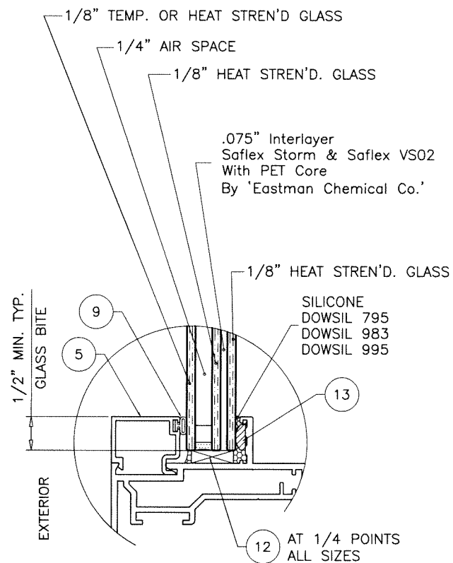
GLASS TYPE 'Ai' 11/16" OVERALL INSUL. LAM. GLASS
